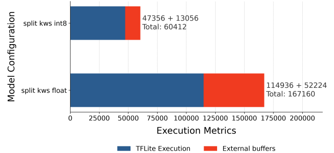
Figure 9: Graph of peak RAM usage of the KWS models
