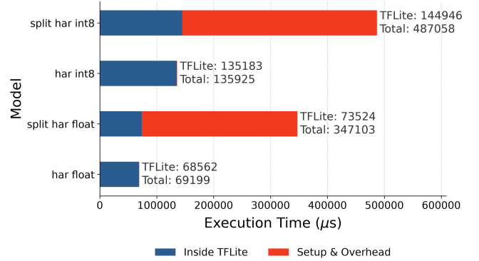
(a) Latency comparison between the HAR models
