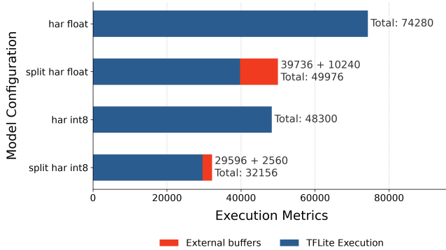
Figure 8: Graph of peak RAM usage of the HAR models
