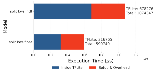
(b) Latency comparison between KWS float32 and int8 models
