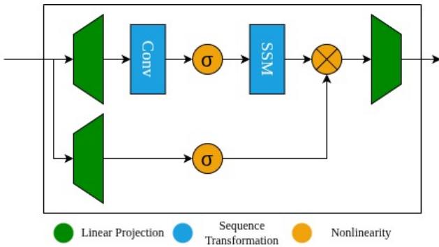
Figure 1: Diagram of the Mamba block
